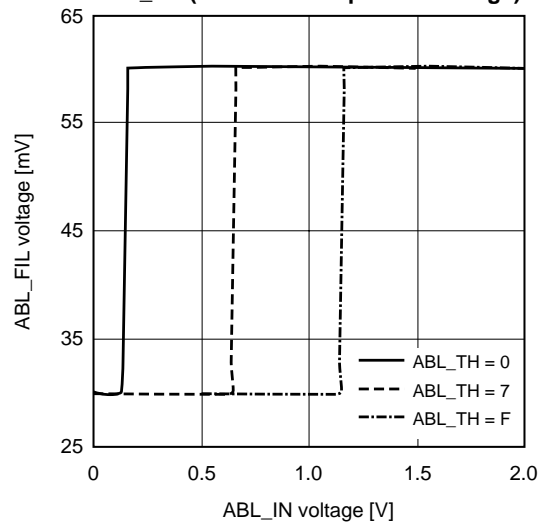
ABL_TH (Threshold in quick discharge)
