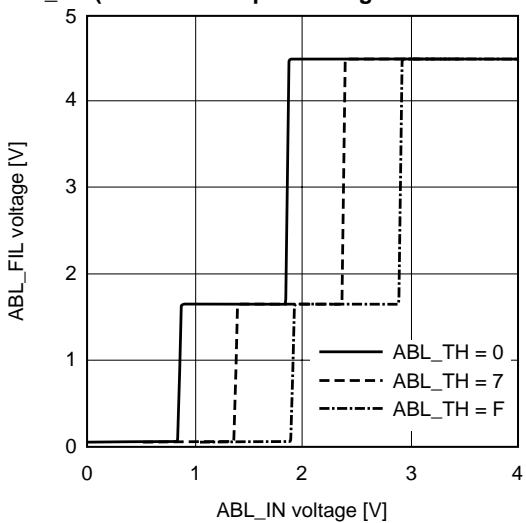
ABL_TH (Threshold in quick charge and normal charge)
